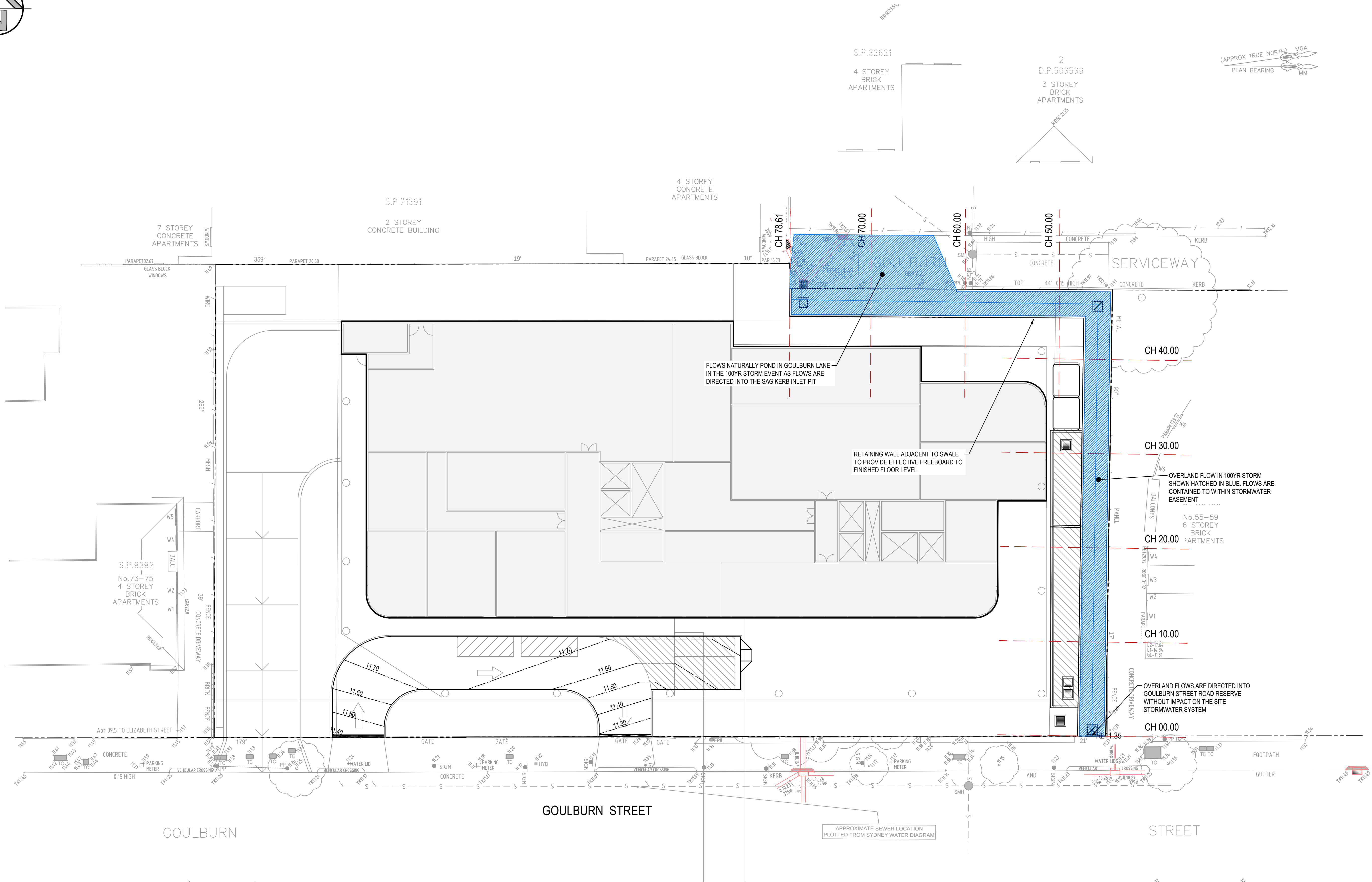
POST-DEVELOPED FLOOD EXTENT PLAN SCALE: 1:200
